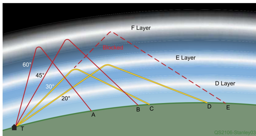
Figure 3 — The ionosphere's E layer blocks low-angle signals.
